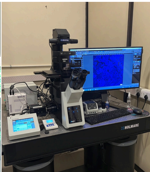
Fluorescence Microscope
